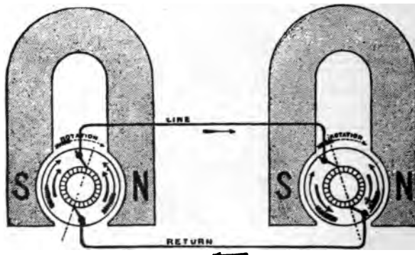
FIG. 988.—Diagram Showing the Operative Conditions of a Dynamo Generator and Electrical Motor. The machine on the left is the dynamo, that on the right the motor.
